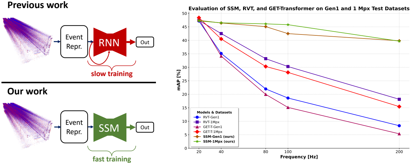
Figure 1. Top-Left Previous works [13, 34] use RNN architectures with convolutional or attention mechanisms to train models that have superior performance on downstream tasks. However, the use of RNNs leads to slower training and the learned weights only generalize well to data deployed at the same frequency as that used at training time. Bottom-Left We solve this problem by utilizing SSMs for temporal aggregation, which enables faster training by either utilizing the S4 model [19] or S5 [41] parallel scans. By their nature, these models allow deployment at different frequencies than those used at training time since they have a learnable timescale parameter. Right Our SSM-based models achieve an average performance drop between training and testing frequencies of 3.31 mAP averaged on both Gen1 [8] and 1 Mpx [34] datasets, while RVT [13] and GET [33] have a drop of 21.25 and 24.53 mAP, respectively.
